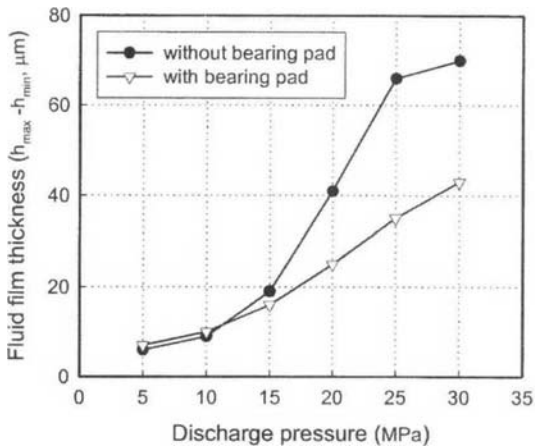
Fig. 13 Difference between maximum and minimum fluid film thickness
