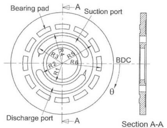
Fig. 4 Shapes of test valve plates
