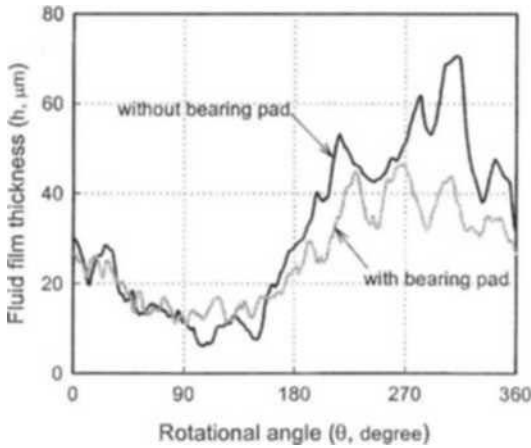
Fig. 11 Comparison of fluid film thickness at 25 MPa
