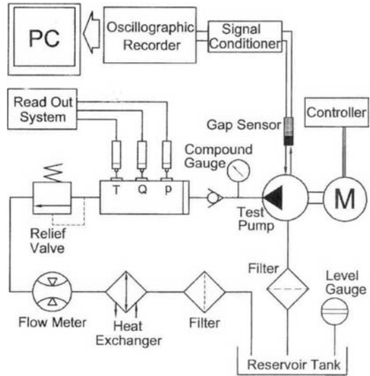
Fig. 5 Hydraulic circuit of measurement system
